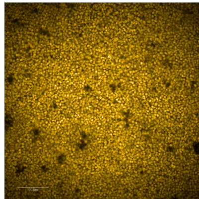
Pax6
