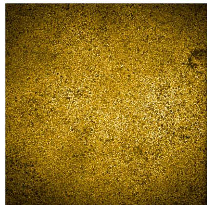
Pax6
